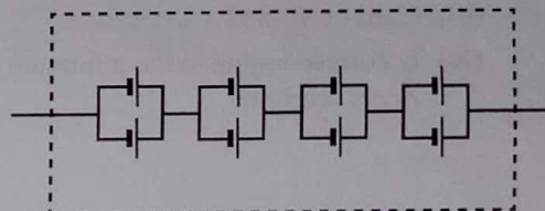
Figure (1): Battery Module
